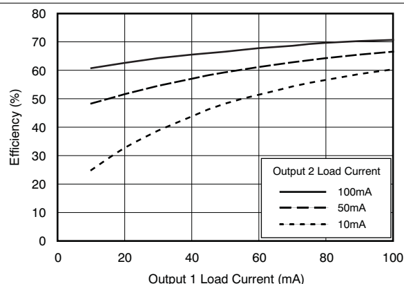
Figure 2. DCH010505D Efficiency
