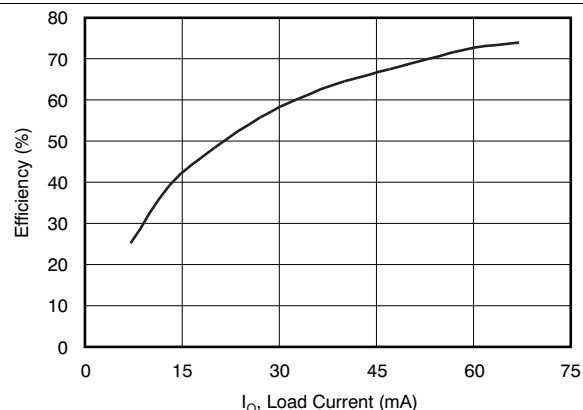
Figure 13. DCH010515S Efficiency
