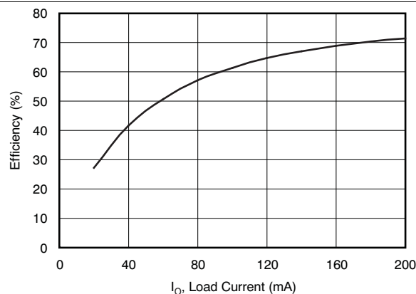
Figure 28. DCH010505S Efficiency
