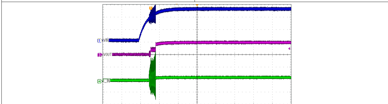
Figure 29. DCP010505BP Start-Up at No Load
