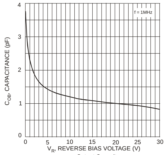
Fig.10 Output Capacitance
