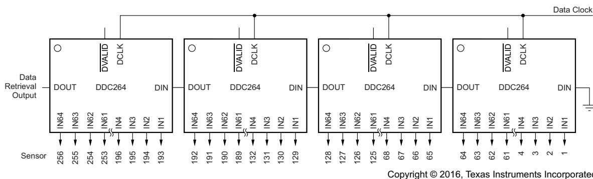
Figure 24. Daisy-Chain DDC264s
