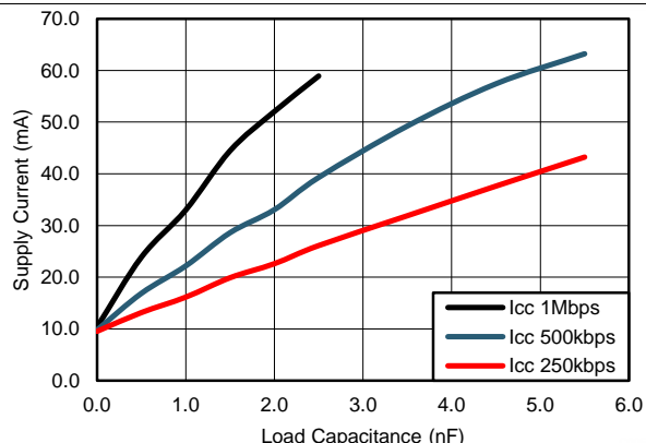
Figure 1. Supply Current vs. Load Capacitance V_{CC} = 3.3\text{ V} , V_L = 1.8\text{ V} , R_{LOAD} = 3\text{ k}\Omega , CH2 = 32\text{ kbps}
