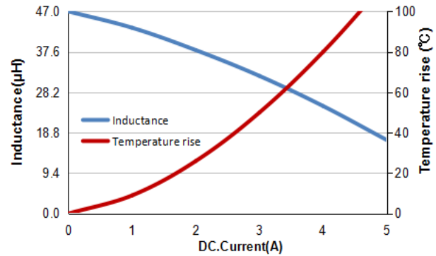
MWSA0605S-470MT
