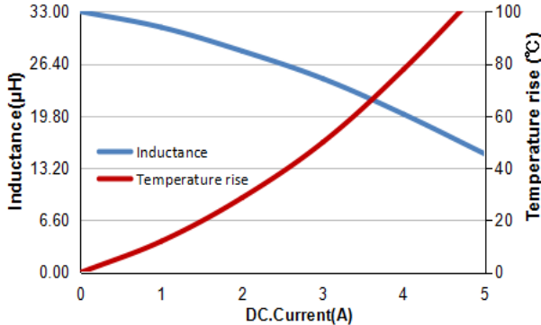
MWSA0605S-330MT
