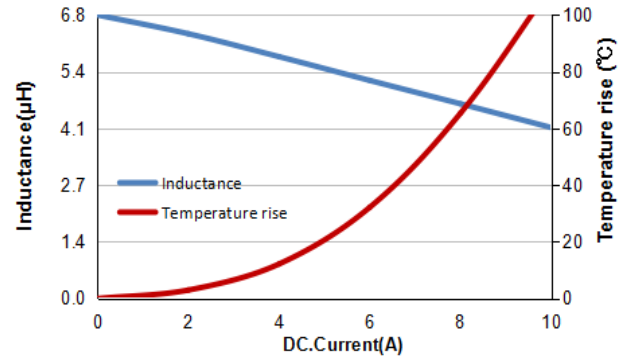
MWSA0605S-6R8MT
