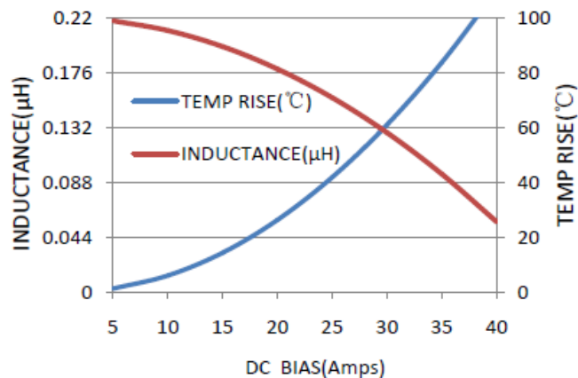
MWSA0618S-R22MT
