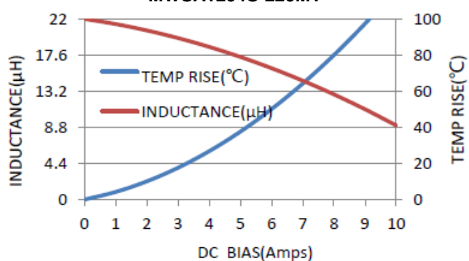
MWSA1204S-220MT
