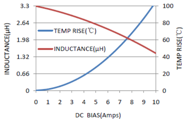
MWSA0503S-3R3MT
