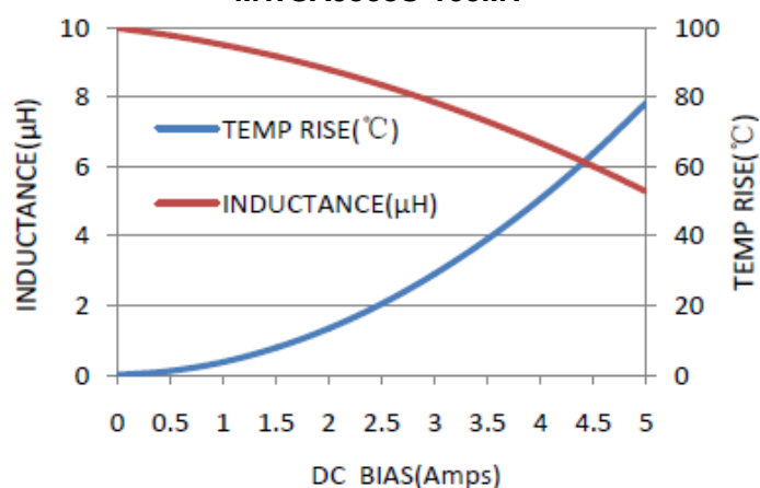
MWSA0503S-100MT
