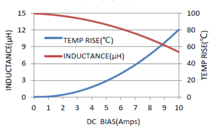
MWSA1204S-150MT
