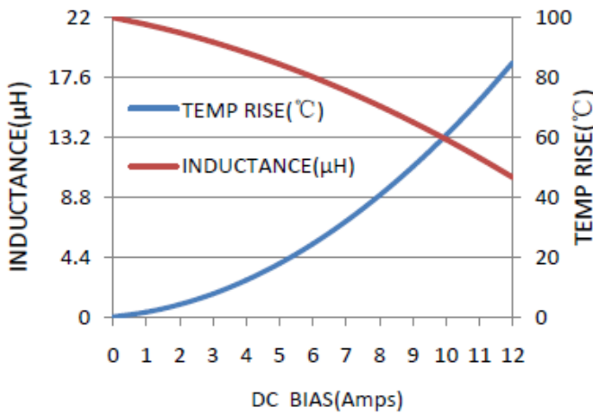
MWSA1206S-220MT
