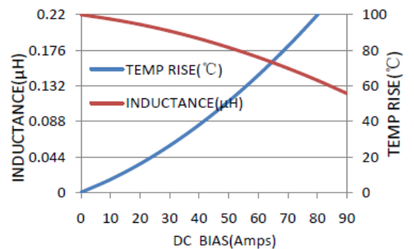
MWSA1004S-R22MT
