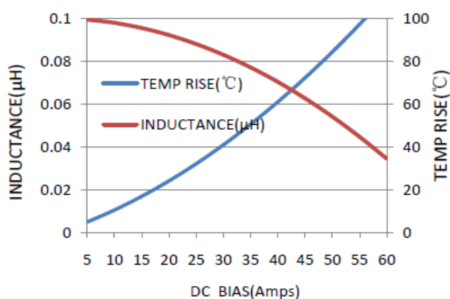
MWSA0618S-R10MT
