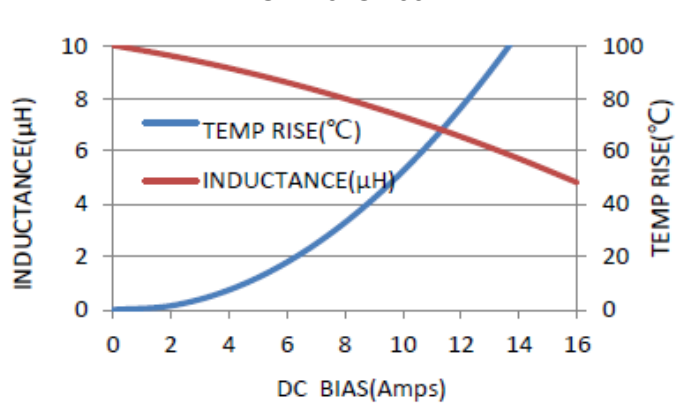
MWSA1204S-100MT
