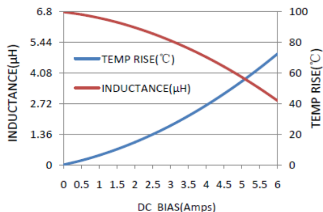
MWSA0503S-6R8MT
