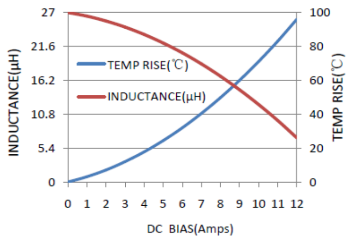
MWSA1206S-270MT
