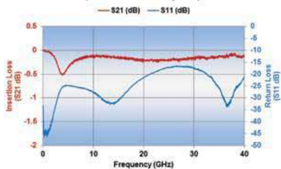
P21BN300MA4282 Opti-Cap Typical Performance (Reference 50 Ohm System)
