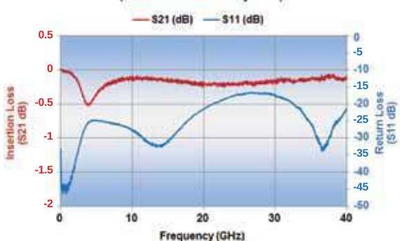
P42BN300MA4679 Opti-Cap Typical Performance (Reference 50 Ohm System)
