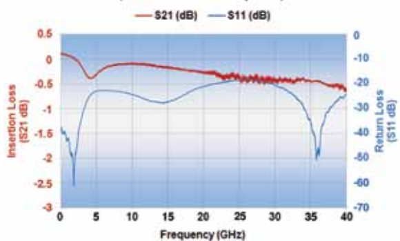
P21BN300MA04733 Opti-Cap Typical Performance (Reference 50 Ohm System)
