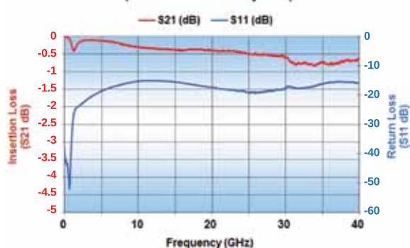
P62BN300MA2636 Opti-Cap Typical Performance (Reference 50 Ohm System)
