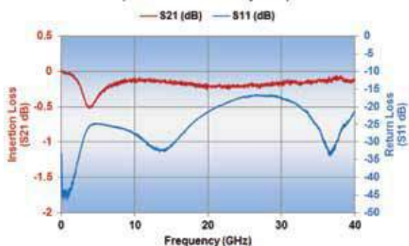
P21BN300MA4572 Opti-Cap Typical Performance (Reference 50 Ohm System)
