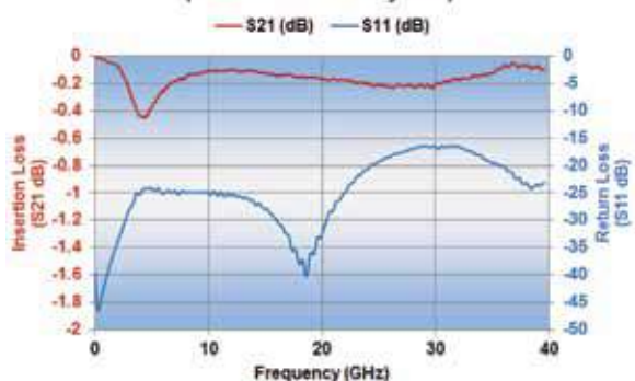
P21BN300MA3976 Opti-Cap Typical Performance (Reference 50 Ohm System)
