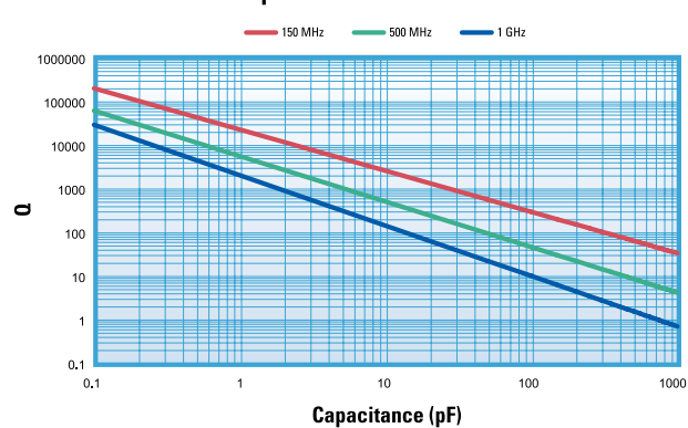
Q vs Capacitance DLI C17 AH Series
