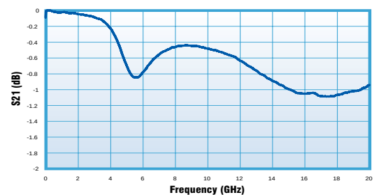
C04BL121X-5UN-X0T Insertion Loss (S21)
