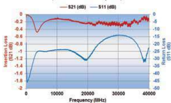
P21BN300MA4678 Opti-Cap Typical Performance (Reference 50 Ohm System)
