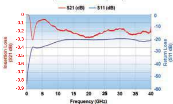
P42BN300MA3182 Opti-Cap Typical Performance (Reference 50 Ohm System)
