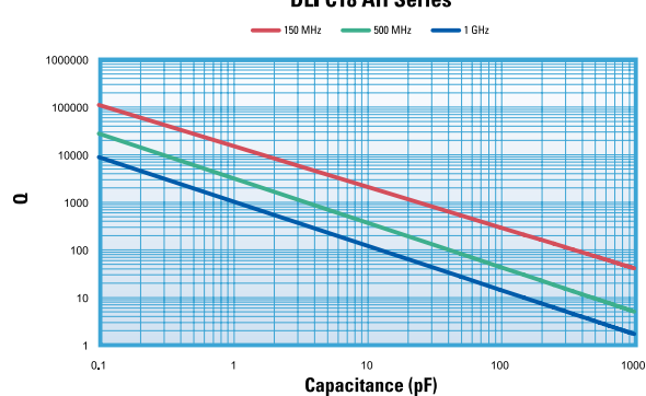
Q vs Capacitance DLI C18 AH Series
