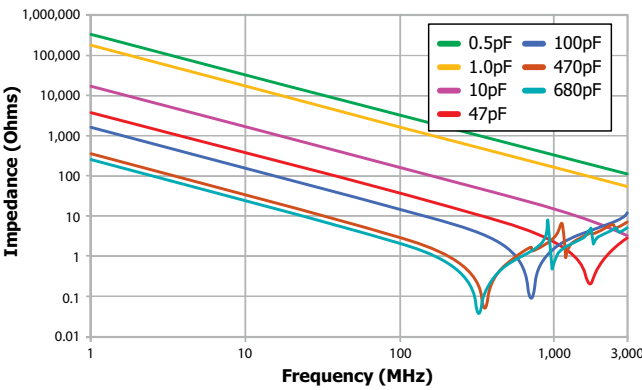
Q Series — Impedance vs. Frequency — Case Size 1111
