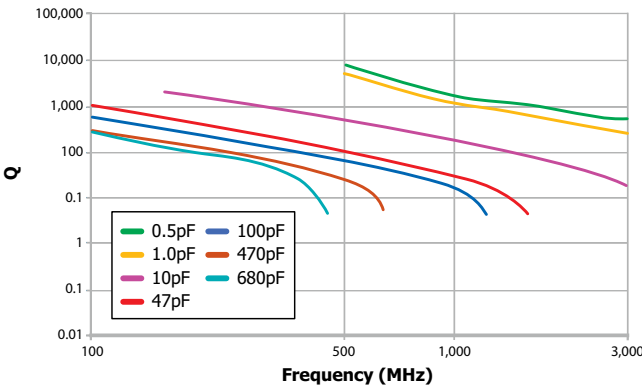
Q Series — Q vs. Frequency — Case Size 1111
