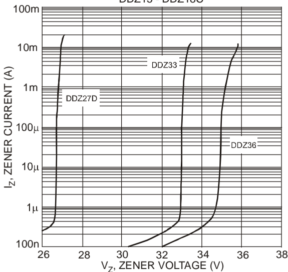
Fig. 8 Typical Zener Breakdown Characteristics, DDZ27D - DDZ36
