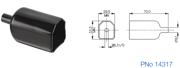
Insulation Boot
