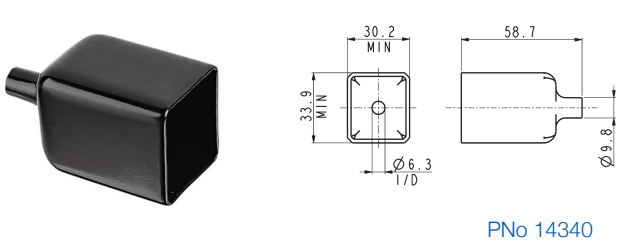
Insulation Boot
