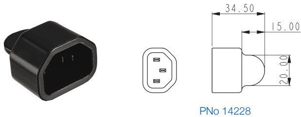
Blanking Cover
