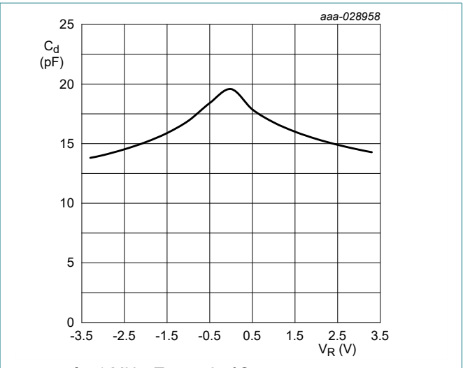
Fig. 4. Diode capacitance as a function of reverse voltage; typical values f = 1\text{ MHz}; T_{amb} = 25\text{ }^{\circ}\text{C}
