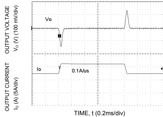
Figure 11. Transient Response to a Dynamic Load Change from 50% to 75% to 50% of full load ( 5\text{V}@15\text{A} ) at V_{in} = 48\text{V} .
