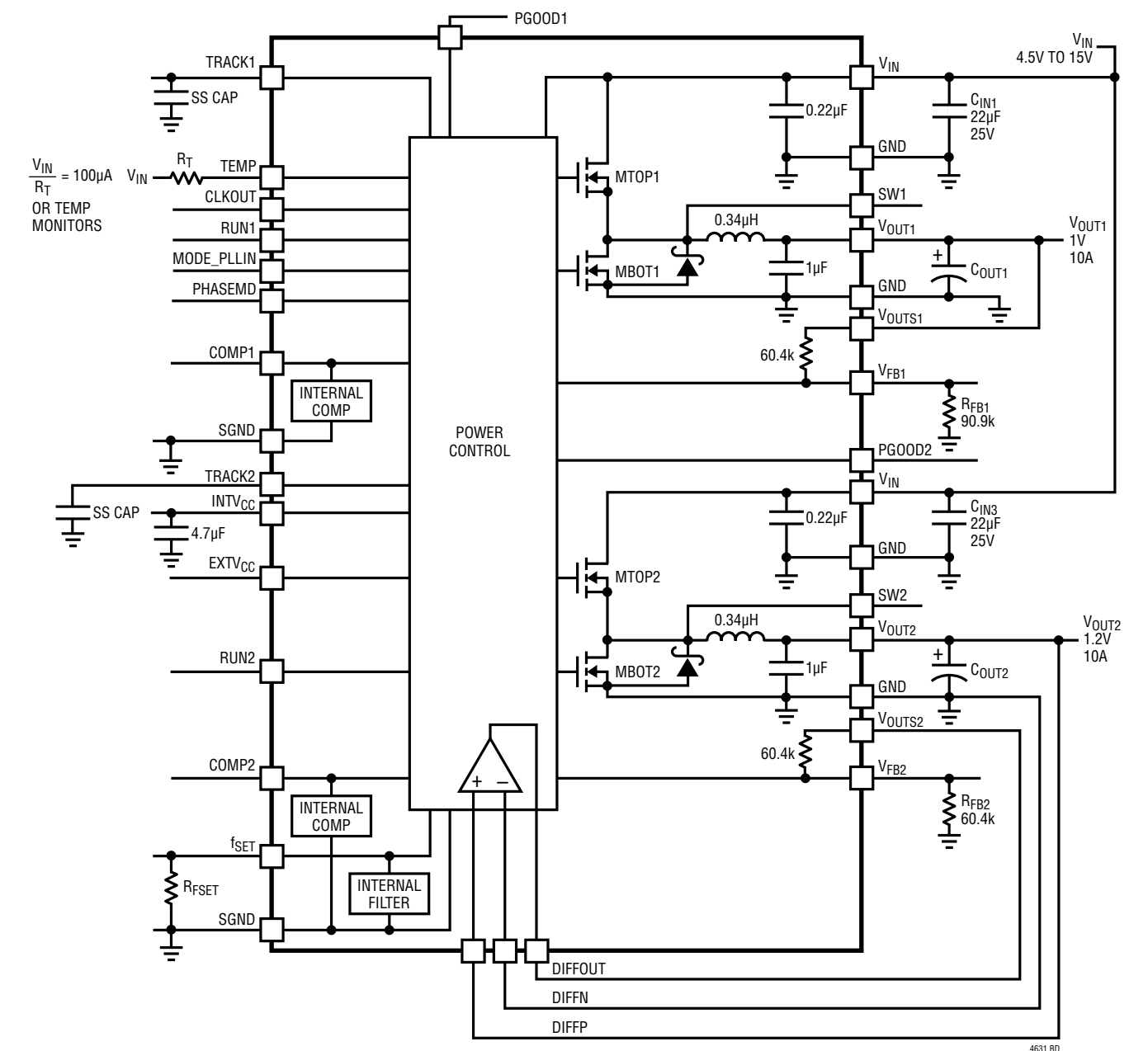
Figure 1. Simplified LTM4631 Block Diagram
