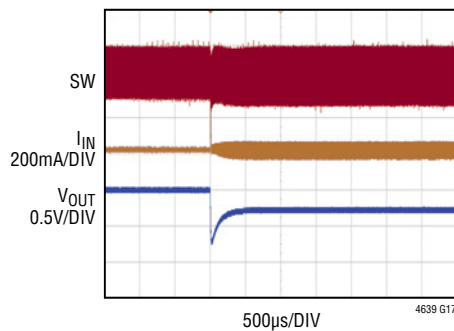
Output Short-Circuit
