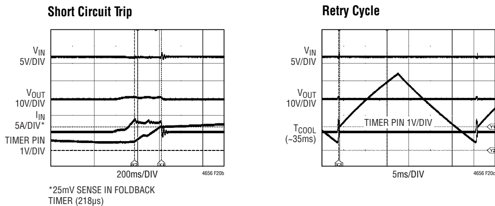
Figure 20. 5V Input to 24V OUT at 1.35A Design
