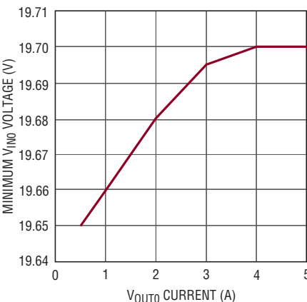
Minimum V_{INO} vs Output Current, V_{OUT0} = 18\text{V}
