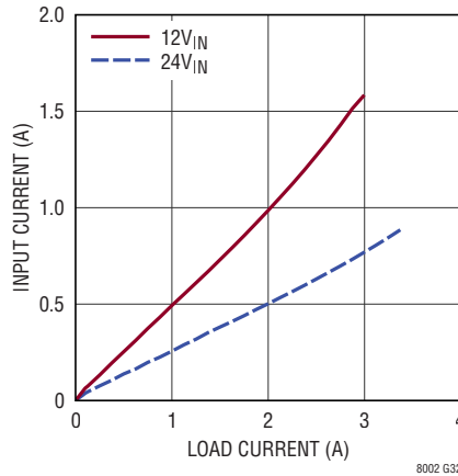
Input vs Load Current, V_{OUT} = -5\text{V}
