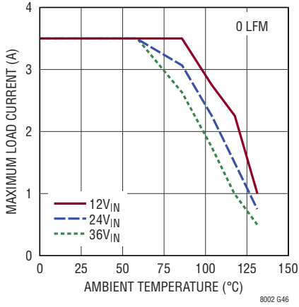
Derating, H-Grade, V_{OUT} = 3.3\text{V} , BIAS = 5V, DC2501A Demo Board
