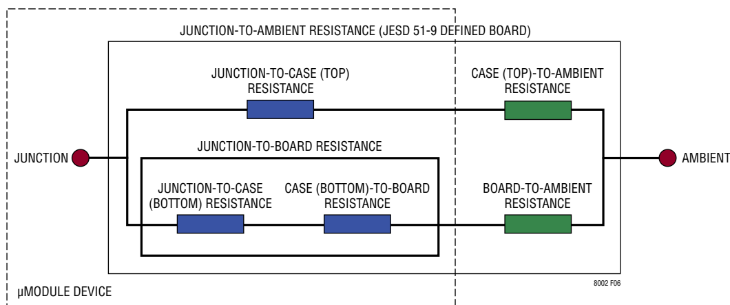
Figure 6. Graphical Representation of the Thermal Resistance Between the Device Junction and Ambient
