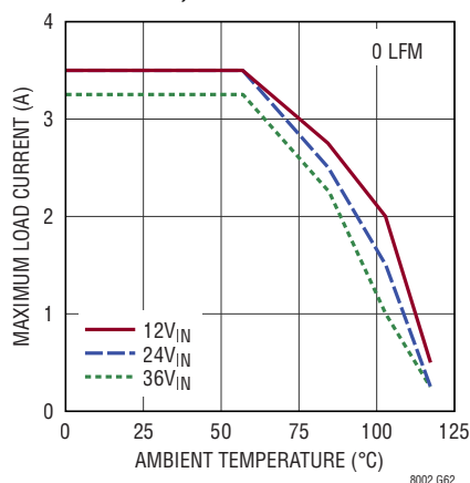
Derating, I-Grade, V_{OUT} = 1.8\text{V} , BIAS = 5V, DC2501A Demo Board
