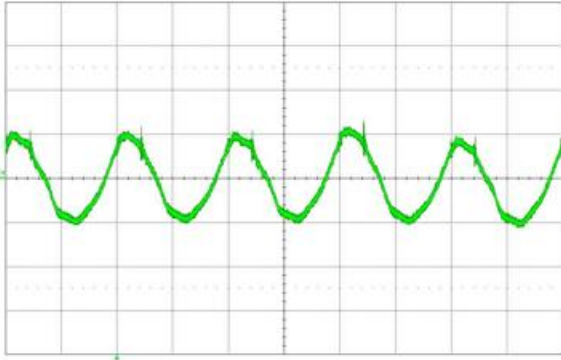
Figure 36. Output voltage ripple (20 mV/div.) at full rated load current into a resistive load with C_o = 10\ \mu\text{F} tantalum + 1\ \mu\text{F} ceramic and V_{in} = 48\ \text{V} . Time scale: 2\ \mu\text{s}/\text{div.}
