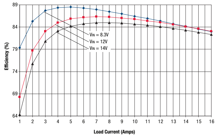
OKX2-T/16-D12 Efficiency vs. Line Voltage and Load Current @ +25°C (V OUT = 1.2V)
