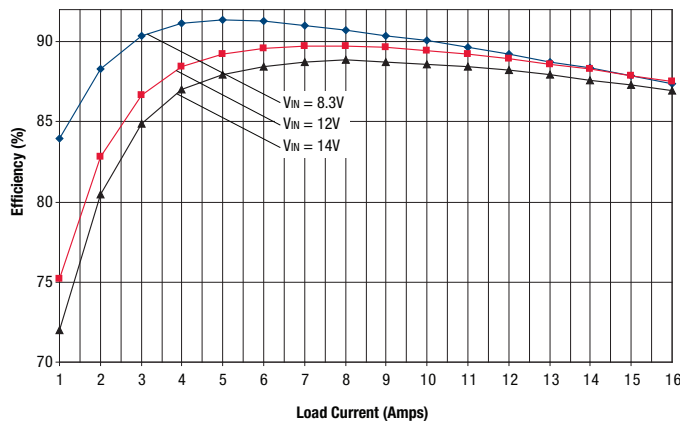
OKX2-T/16-D12 Efficiency vs. Line Voltage and Load Current @ +25°C ( V_{OUT} = 2.5V )
