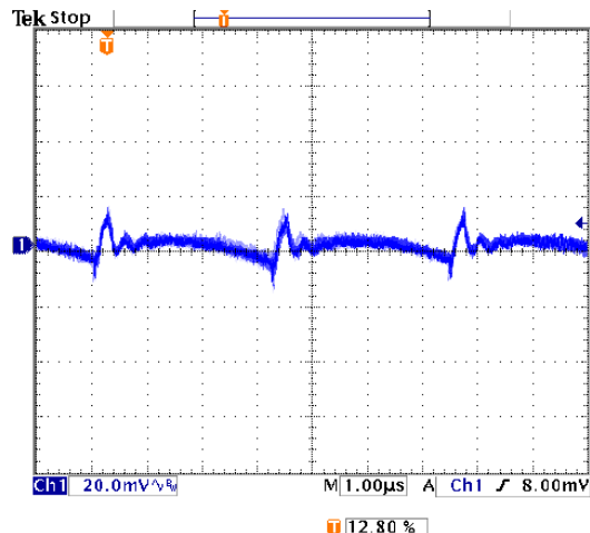
OKX2-T/16-D12 Output Ripple and Noise ( V_{IN}=12V, V_{OUT}=0.75V, I_{OUT}=16A, C_{IN}=1000\mu F , Load=1 \mu F // 10 \mu F , ScopeBW=100MHz)
