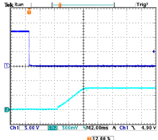
OKX2-T/16-D12-C On/Off Enable Startup Delay ( V_{IN}=12V, V_{OUT}=0.75V, I_{OUT}=16A, C_{IN}=1000\mu F , Load=1 \mu F // 10 \mu F ) Trace 1=Enable In, Trace2=Vout
