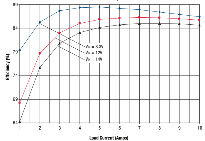
OKX2-T/10-D12 Efficiency vs. Line Voltage and Load Current @ +25°C ( V_{OUT} = 1.2V )
