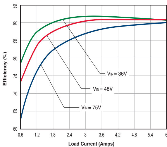
UVQ-18/6-D48N Efficiency vs. Line Voltage and Load Current @ 25°C
