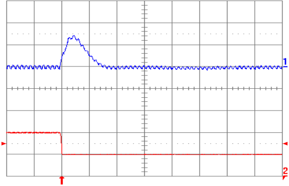
Fig. 2.0V.8: Output voltage response for V_{out} = 2.0\text{ V} to negative load current step change from 10 A to 5 A with slew rate of -5 A/μs at V_{in} = 5\text{ V} . Top trace: output voltage (100 mV/div.); Bottom trace: load current (5 A/div.). C_o = 47\text{ }\mu\text{F} ceramic + 1 μF ceramic. Time scale: 20 μs/div.
