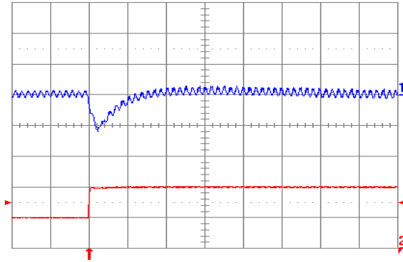
Fig. 3.3V.7: Output voltage for V_{out} = 3.3\text{ V} to positive load current step change from 5 A to 10 A with slew rate of 5\text{ A}/\mu\text{s} at V_{in} = 5\text{ V} . Top trace: output voltage (100 mV/div.); Bottom trace: load current (5 A/div.). C_o = 47\text{ }\mu\text{F} ceramic + 1\text{ }\mu\text{F} ceramic. Time scale: 20\text{ }\mu\text{s}/\text{div} .
