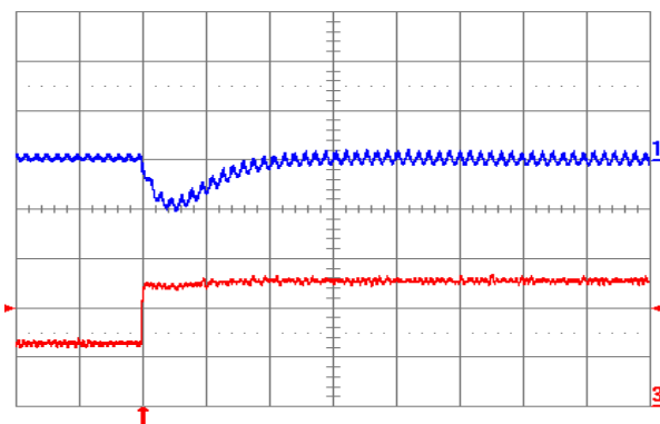
Fig. 1.0V.7: Output voltage response V_{out} = 1.0 V to positive load current step change from 5 A to 10 A with slew rate of 5\text{ A}/\mu\text{s} at V_{in} = 5 V. Top trace: output voltage (100 mV/div.); Bottom trace: load current (5 A/div.). C_o = 47\text{ }\mu\text{F} ceramic + 1\text{ }\mu\text{F} ceramic. Time scale: 20\text{ }\mu\text{s}/\text{div} .
