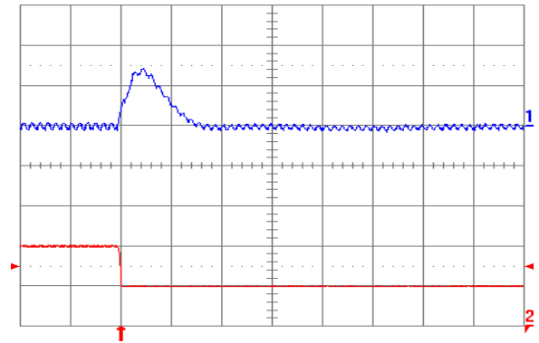
Fig. 1.8V.8: Output voltage response for V_{out} = 1.8 V to negative load current step change from 10 A to 5 A with slew rate of -5\text{ A}/\mu\text{s} at V_{in} = 5 V. Top trace: output voltage (100 mV/div.); Bottom trace: load current (5 A/div.). C_o = 47\text{ }\mu\text{F} ceramic + 1\text{ }\mu\text{F} ceramic. Time scale: 20\text{ }\mu\text{s/div.}
