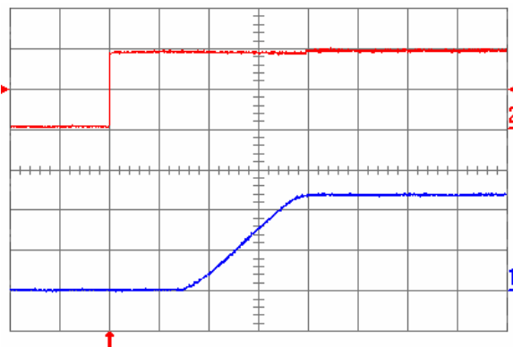
Fig. 1.2V.5: Turn-on transient for V_{out} = 1.2 V with the application of Enable signal at full rated load current (resistive) and 47 \mu\text{F} external capacitance at V_{in} = 5 V. Top trace: Enable signal (2 V/div.); Bottom trace: output voltage (500 mV/div.); Time scale: 2 ms/div.
