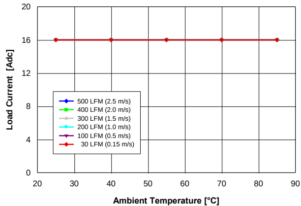
Fig. 1.2V.1: Available load current vs. ambient temperature and airflow rates for V_{out} = 1.2 V converter mounted vertically with V_{in} = 5 V, and maximum MOSFET temperature \leq 120 °C.
