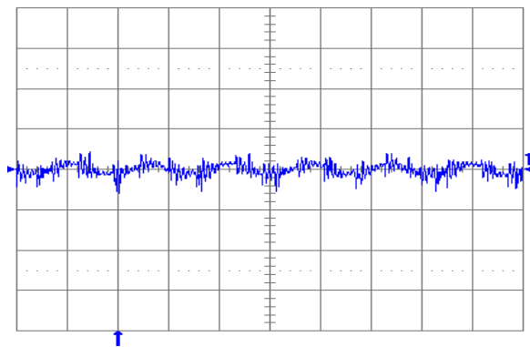
Fig. 1.5V.6: Output voltage ripple (20 mV/div.) at full rated load current into a resistive load with external capacitance 47\text{ }\mu\text{F} ceramic + 1\text{ }\mu\text{F} ceramic, and V_{in} = 5\text{ V} for V_{out} = 1.5\text{ V} . Time scale: 2 µs/div.
