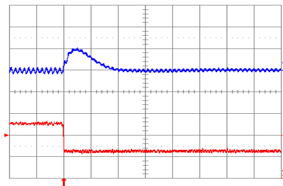
Fig. 1.0V.8: Output voltage response for V_{out} = 1.0 V to negative load current step change from 10 A to 5 A with slew rate of -5\text{ A}/\mu\text{s} at V_{in} = 5 V. Top trace: output voltage (100 mV/div.); Bottom trace: load current (5 A/div.). C_o = 47\text{ }\mu\text{F} ceramic + 1\text{ }\mu\text{F} ceramic. Time scale: 20\text{ }\mu\text{s}/\text{div} .
