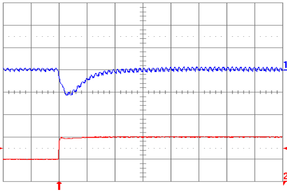
Fig. 1.8V.7: Output voltage response for V_{out} = 1.8 V to positive load current step change from 5 A to 10 A with slew rate of 5\text{ A}/\mu\text{s} at V_{in} = 5 V. Top trace: output voltage (100 mV/div.); Bottom trace: load current (5 A/div.). C_o = 47\text{ }\mu\text{F} ceramic + 1\text{ }\mu\text{F} ceramic. Time scale: 20\text{ }\mu\text{s/div.}
