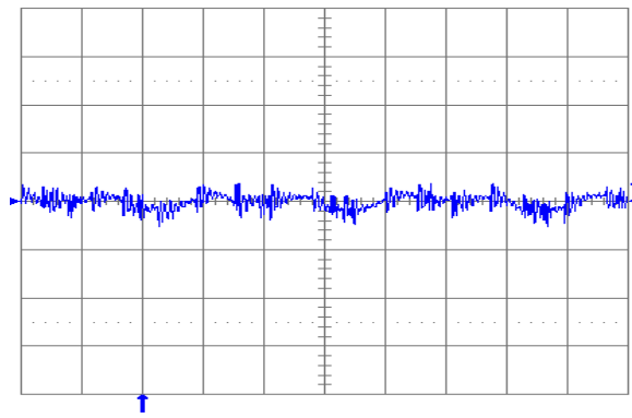
Fig. 1.0V.6: Output voltage ripple (20 mV/div.) at full rated load current into a resistive load with external capacitance 47\text{ }\mu\text{F} ceramic + 1\text{ }\mu\text{F} ceramic, and V_{in} = 5 V for V_{out} = 1.0 V. Time scale: 2\text{ }\mu\text{s}/\text{div} .
