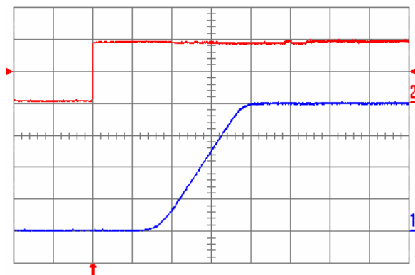
Fig. 2.0V.5: Turn-on transient for V_{out} = 2.0 V with the application of Enable signal at full rated load current (resistive) and 47 \mu\text{F} external capacitance at V_{in} = 5 V. Top trace: Enable signal (2 V/div.); Bottom trace: output voltage (500 mV/div.); Time scale: 2 ms/div.
