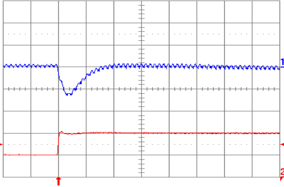
Fig. 1.2V.6: Output voltage response for V_{out} = 1.2\text{ V} to positive load current step change from 5 A to 10 A with slew rate of 5\text{ A}/\mu\text{s} at V_{in} = 5\text{ V} . Top trace: output voltage (100 mV/div.); Bottom trace: load current (5 A/div.). C_o = 47\text{ }\mu\text{F} ceramic + 1\text{ }\mu\text{F} ceramic. Time scale: 20\text{ }\mu\text{s}/\text{div} .
