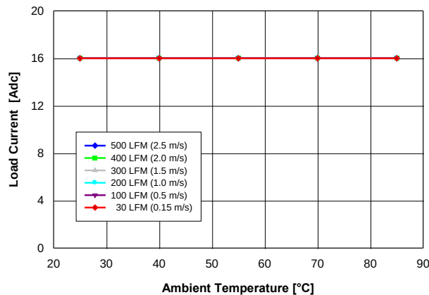
Fig. 1.5V.1: Available load current vs. ambient temperature and airflow rates for V_{out} = 1.5 V converter mounted vertically with V_{in} = 5 V, and maximum MOSFET temperature \leq 120\text{ }^{\circ}\text{C} .
