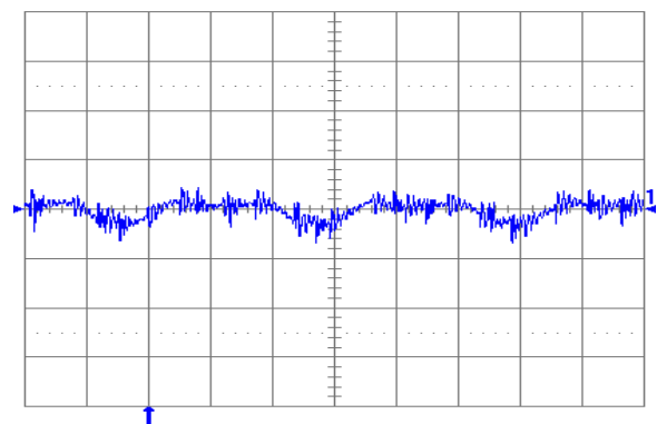
Fig. 1.2V.6: Output voltage ripple (20 mV/div.) at full rated load current into a resistive load with external capacitance 47 \mu\text{F} ceramic + 1 \mu\text{F} ceramic, and V_{in} = 5 V for V_{out} = 1.2 V. Time scale: 2 μs/div.
