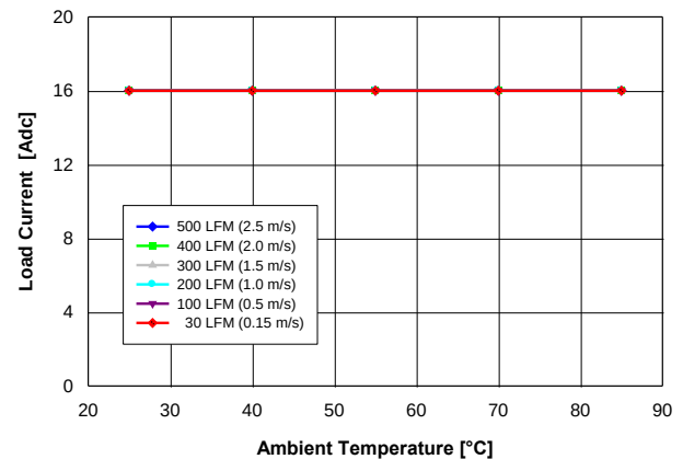
Fig. 1.5V.2: Available load current vs. ambient temperature and airflow rates for V_{out} = 1.5 V converter mounted horizontally with V_{in} = 5 V, and maximum MOSFET temperature \leq 120\text{ }^{\circ}\text{C} .
