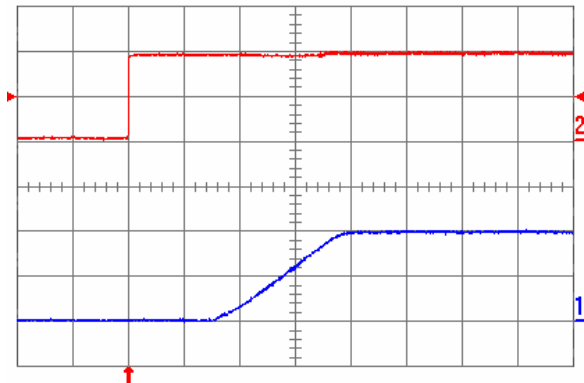
Fig. 1.0V.5: Turn-on transient for V_{out} = 1.0 V with the application of Enable signal at full rated load current (resistive) and 47\text{ }\mu\text{F} external capacitance at V_{in} = 5 V. Top trace: Enable signal (2 V/div.); Bottom trace: output voltage (500 mV/div.); Time scale: 2 ms/div.
