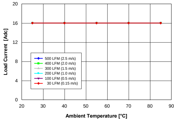
Fig. 3.3V.1: Available load current vs. ambient temperature and airflow rates for V_{out} = 3.3 V converter mounted vertically with V_{in} = 5 V, and maximum MOSFET temperature \leq 120 °C.
