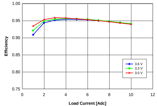
Fig. 2.5V.4: Efficiency vs. load current and input voltage for V_{out} = 2.5\text{ V} converter mounted horizontally with air flowing at a rate of 200 LFM (1 m/s) and T_a = 25\text{ }^{\circ}\text{C} .
