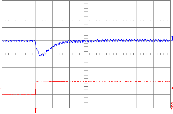
Fig. 2.0V.7: Output voltage response for V_{out} = 2.0\text{ V} to positive load current step change from 5 A to 10 A with slew rate of 5 A/μs at V_{in} = 5\text{ V} . Top trace: output voltage (100 mV/div.); Bottom trace: load current (5 A/div.). C_o = 47\text{ }\mu\text{F} ceramic + 1 μF ceramic. Time scale: 20 μs/div.
