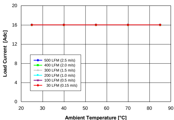
Fig. 0.7525V.1: Available load current vs. ambient temperature and airflow rates for V_{out} = 0.7525 V converter mounted vertically with V_{in} = 5 V, and maximum MOSFET temperature \leq 120\text{ }^{\circ}\text{C} .
