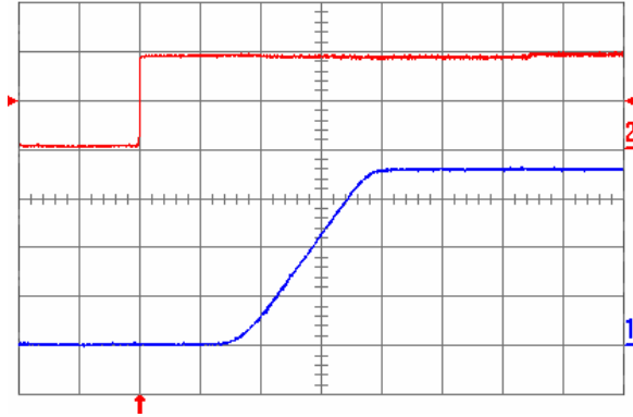
Fig. 1.8V.5: Turn-on transient for V_{out} = 1.8 V with the application of Enable signal at full rated load current (resistive) and 47\text{ }\mu\text{F} external capacitance at V_{in} = 5 V. Top trace: Enable signal (2 V/div.); Bottom trace: output voltage (500 mV/div.); Time scale: 2 ms/div.
