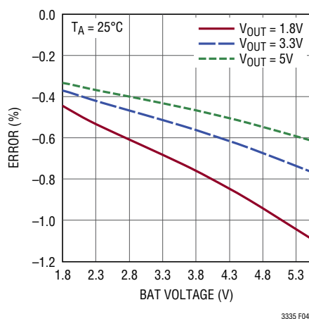
Figure 4. Typical Error Due to Input Quiescent Current for 250mA I_{PEAK} Setting
