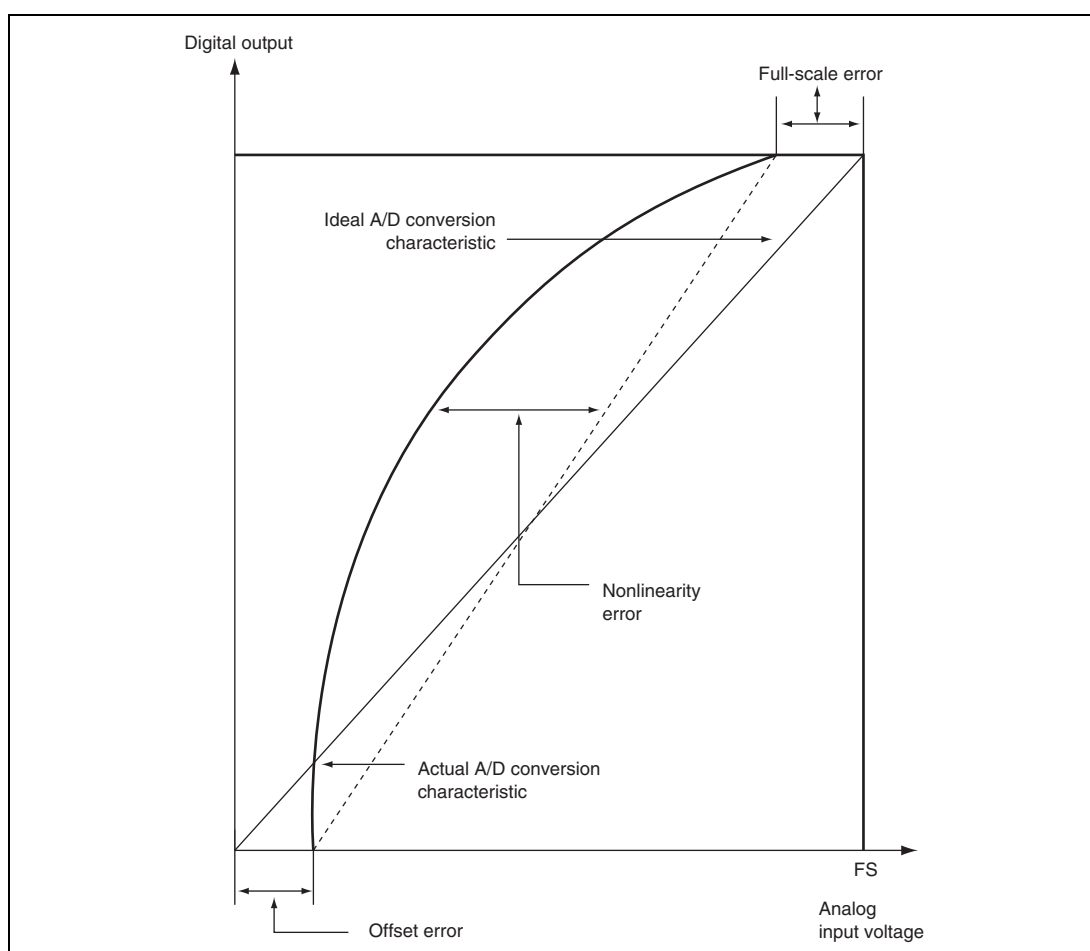
Figure 19.4 A/D Conversion Accuracy Definitions (2)
