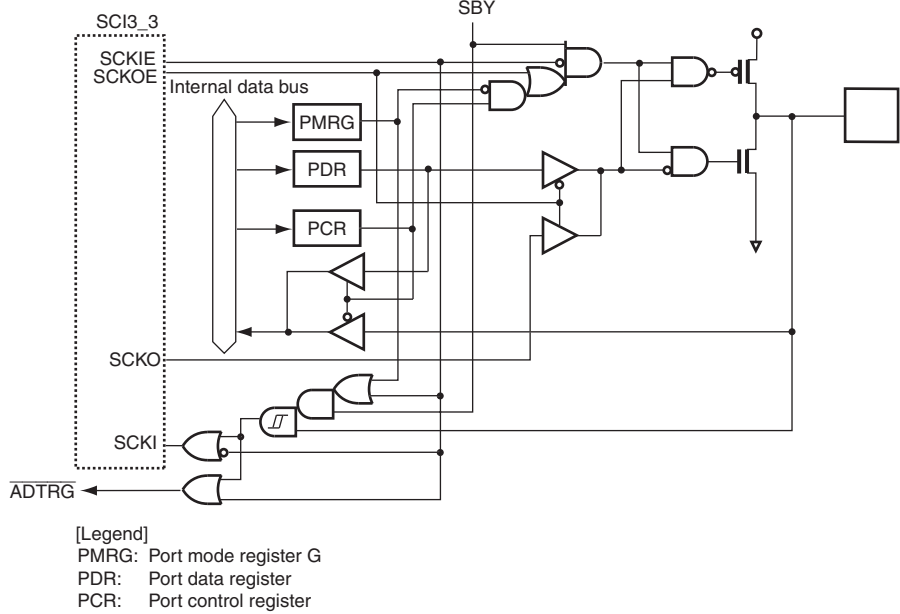
Figure B.32 Port H Block Diagram (PH0)
