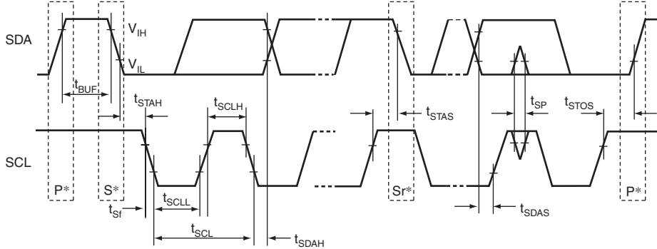
Figure 23.3 Input Timing
