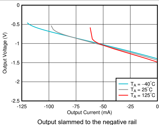
Figure 7-32. Output Swing vs Sinking Current
