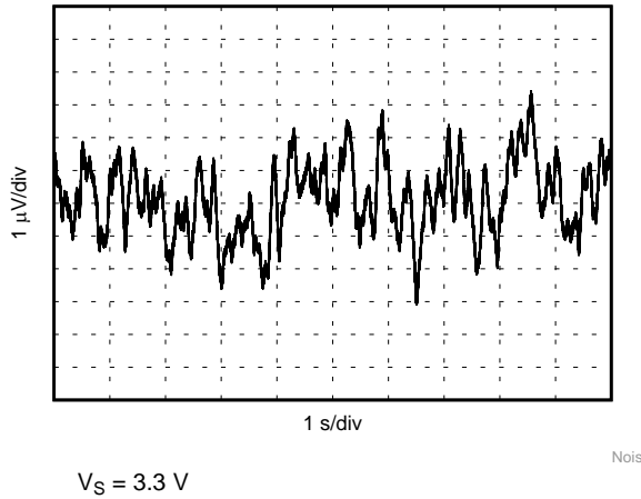
Figure 27. 0.1-Hz to 10-Hz Noise, V_S = 3.3\text{ V}
