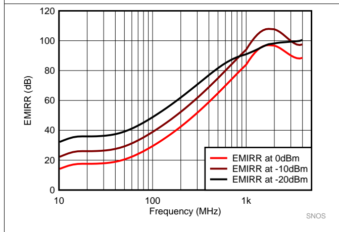
Figure 23. EMIRR Performance
