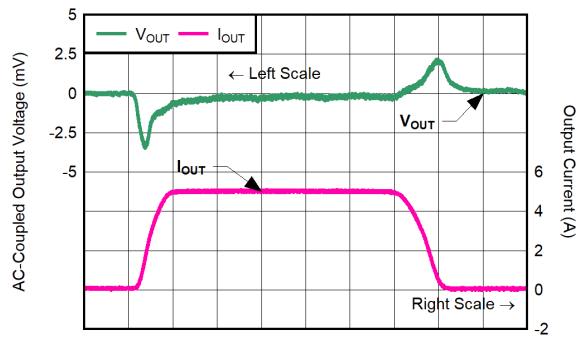
Figure 6-34. Load Transient for V_{OUT} = 0.5 V, I_{OUT} = 100 mA to 5 A, CP Enabled
