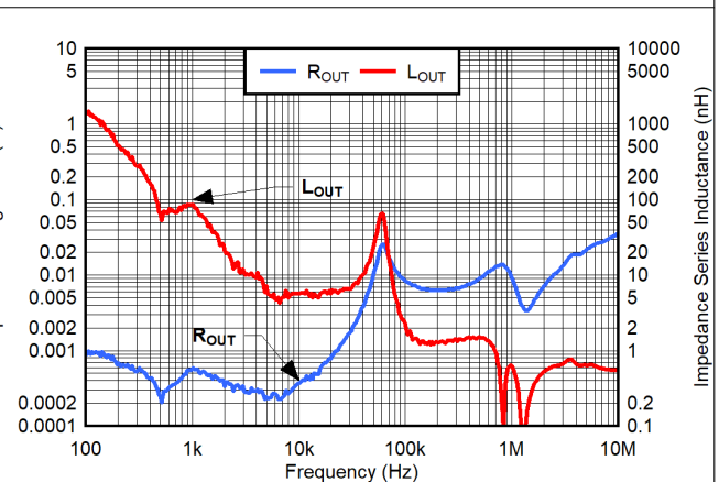
Figure 8-17. V_{IN} = 0.9 V, V_{BIAS} = 3 V, V_{OUT} = 0.5 V, CP\_EN = 0, I_{OUT} = 4.6 A
