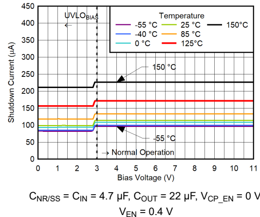
Figure 6-206. IN Pin Shutdown Current vs V_{BIAS} for V_{IN} = 6 V, V_{OUT(nom)} = 0.5 V, CP Disabled
