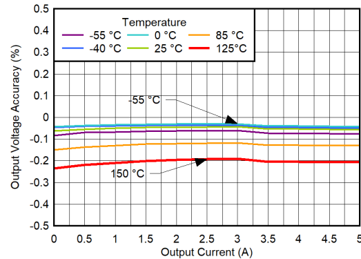
Figure 6-116. Output Voltage Accuracy vs I_{OUT} for V_{IN} = 6 V, V_{BIAS} = 3 V, CP Enabled
