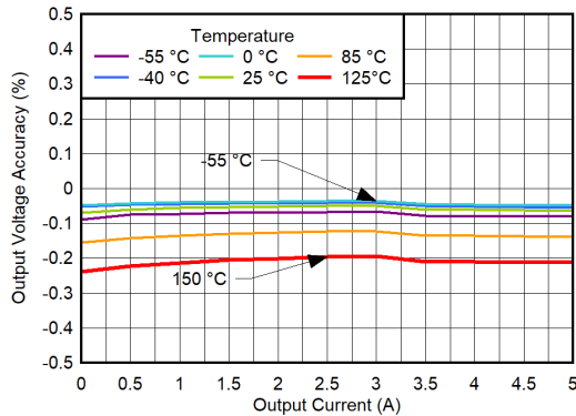
Figure 6-115. Output Voltage Accuracy vs I_{OUT} for V_{IN} = 6 V, V_{BIAS} = 11 V, CP Enabled
