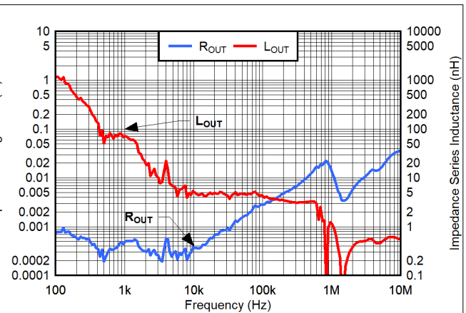
Figure 8-15. V_{IN} = 5.5 V, V_{OUT} = 5 V, V_{BIAS} = 8 V, CP\_EN = 0, I_{OUT} = 500 mA
