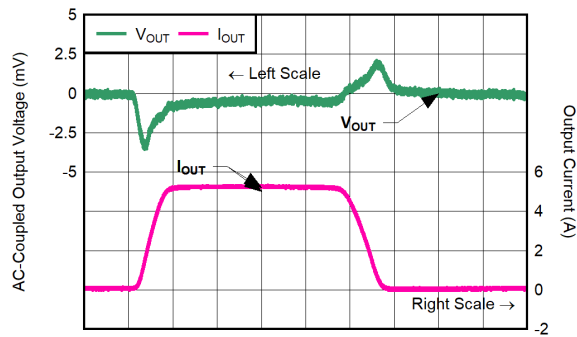
Figure 6-33. Load Transient for V_{OUT} = 0.5 V, I_{OUT} = 100 mA to 5 A, CP Enabled
