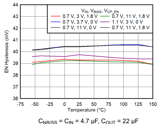
Figure 6-210. EN Hysteresis vs Temperature for V_{IN} = 0.7 V and 1.1 V, V_{OUT} = 0.5 V
