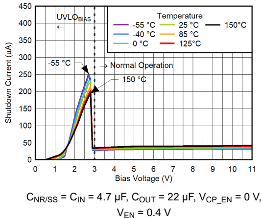
Figure 6-205. BIAS Pin Shutdown Current vs V_{BIAS} for V_{IN} = 6 V, V_{OUT(nom)} = 0.5 V, CP Disabled
