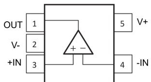
Figure 5-1. LMV321A DBV Package, 5-Pin SOT-23 (Top View)
