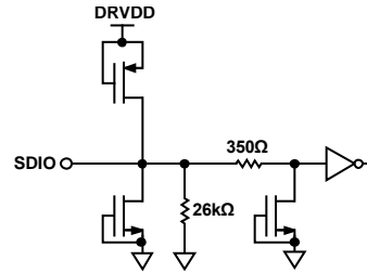
Figure 43. Equivalent SDIO Circuit
