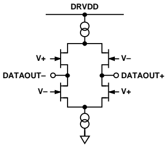
Figure 42. Equivalent LVDS Output Circuit
