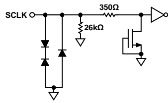
Figure 44. Equivalent SCLK Input Circuit
