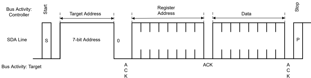
Figure 7-26. Serial Control Bus — WRITE
