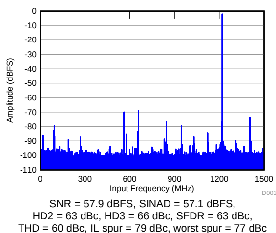
Figure 273. FFT for 1780-MHz Input Frequency
