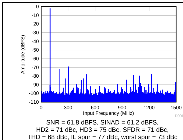
Figure 272. FFT for 100-MHz Input Frequency
