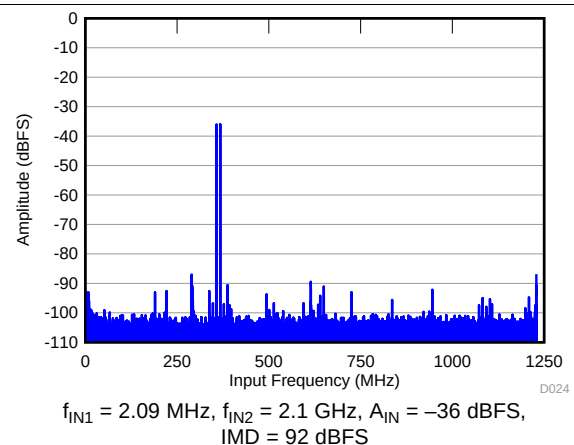
Figure 26. FFT for Two-Tone Input Signal (-36 dBFS, f_s = 2457.6 MSPS)
