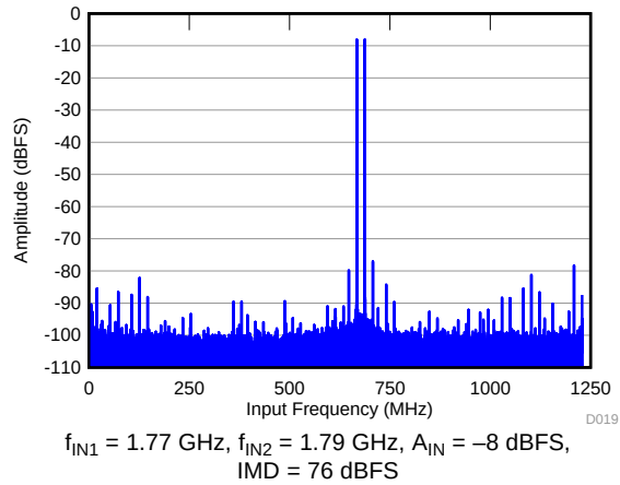
Figure 21. FFT for Two-Tone Input Signal (-8 dBFS, f_s = 2457.6 MSPS)
