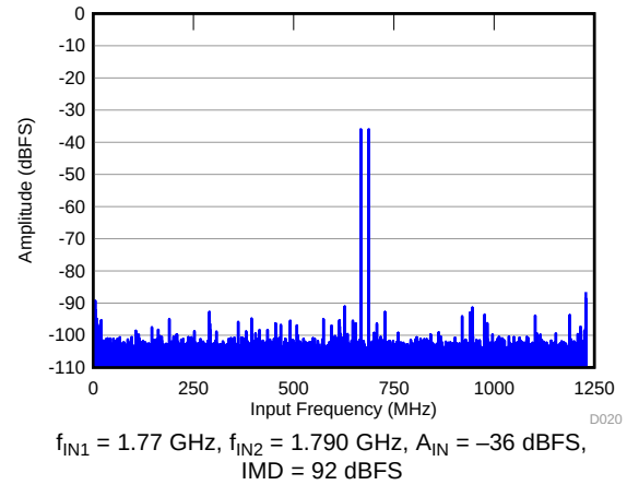
Figure 22. FFT for Two-Tone Input Signal (-36 dBFS, f_s = 2457.6 MSPS)
