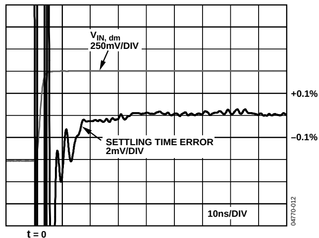
Figure 17. Settling Time (0.1%)
