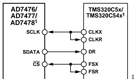
1 ADDITIONAL PINS OMITTED FOR CLARITY Figure 26. Interfacing to the TMS320C5x/C54x
