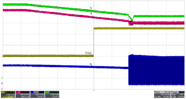
Figure 31. OVP1 Release at V_{\text{FB}} \leq 110\% V_{\text{REF}}
