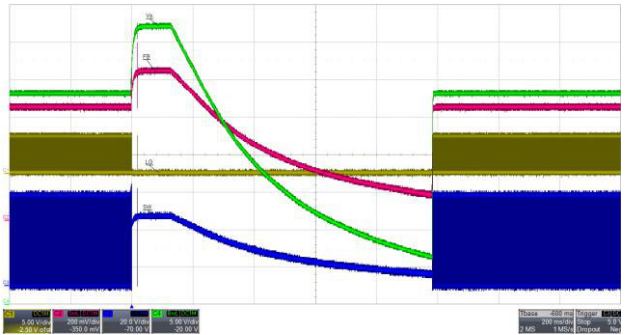
Figure 33. OVP2 Release at V_{\text{FB}} \leq 100\% V_{\text{REF}}
