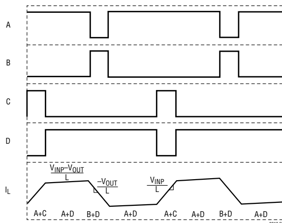
Figure 6. Buck-Boost Region Switching Waveforms
