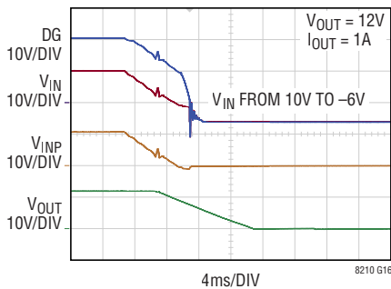
Dynamic Reverse Input Protection (Figure 36)
