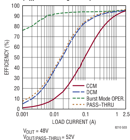
Efficiency vs Load Current ( V_{IN} = 70V – Figure 37)
