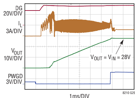
Pass-Thru Start-Up: V_{IN} in Pass-Thru Window (Figure 38)
