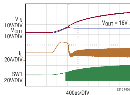
Pass-Thru Positive Surge
