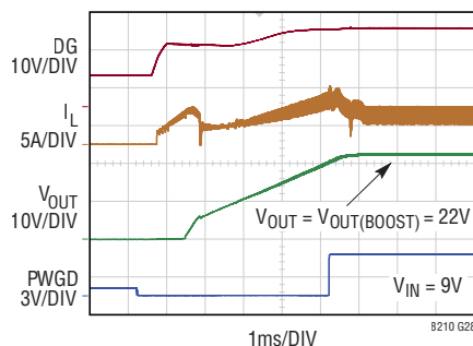
Pass-Thru Start-Up: V_{IN} Below Pass-Thru Window (Figure 38)
