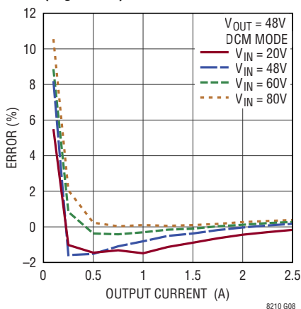
IMON Measurement Accuracy (Figure 37)
