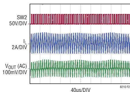
FIGURE 37 CIRCUIT V_{IN} = 20V
