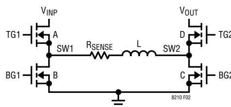
Figure 2. Simplified Diagram of the Power Switches
