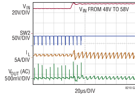
Line Step (Buck-Boost Region – Figure 37)
