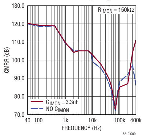
IMON CMRR vs Frequency
