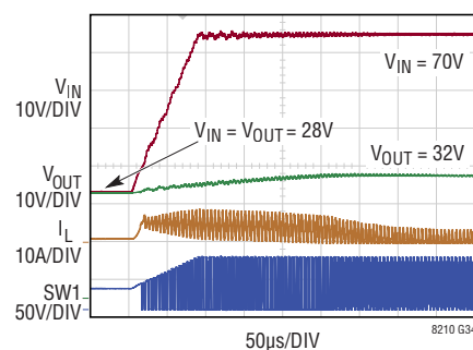
Pass-Thru Positive Surge (Figure 38)
