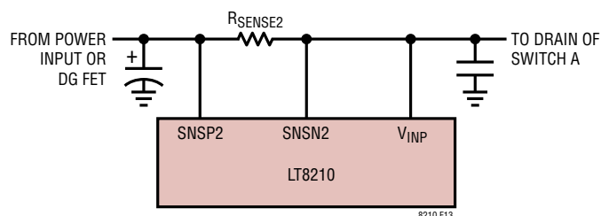
Figure 13. Input Current Sense
