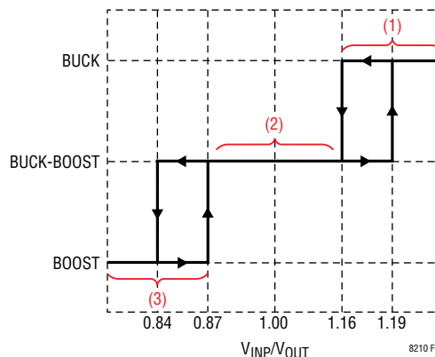
Figure 3. Switching Region vs V_{INP}/V_{OUT} Ratio
