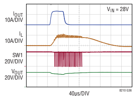
Pass-Thru Current Limit (Figure 38)
