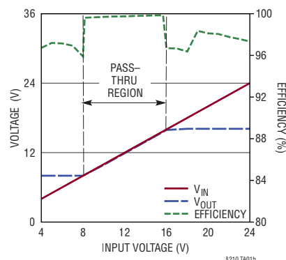
Pass-Thru Transfer Characteristic ( V_{OUT(BOOST)} = 8V , V_{OUT(BUCK)} = 16V )
