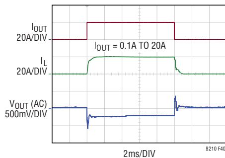
Pass-Thru Load Step
