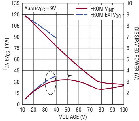
GATEV CC Max Current vs Voltage
