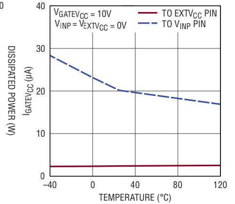
GATEV CC Backdrive Current
