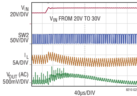
Line Step (Boost Region – Figure 37)
