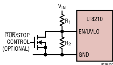
Figure 30. V_{IN} UVLO Implementation Using the EN/UVLO Pin
