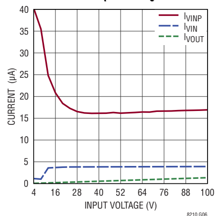
Pass-Thru Non-Switching Currents vs Input Voltage
