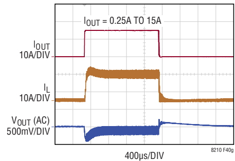
Load Step (V IN = 18V)
