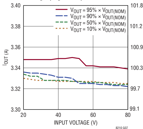
IMON Current Limit vs Input Voltage (Figure 37)
