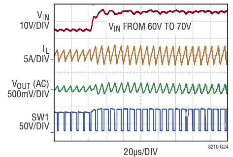
Line Step (Buck Region – Figure 37)
