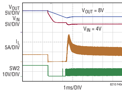
Pass-Thru Negative Surge
