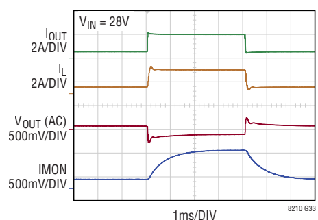
Pass-Thru Load Step (Figure 38)
