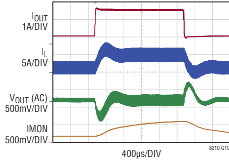
Load Step (Boost Region – Figure 37)
