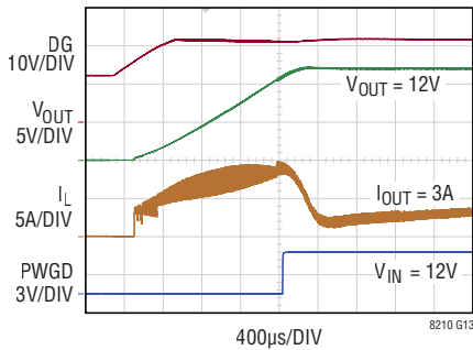
Start-Up (CCM Mode – Figure 36)
