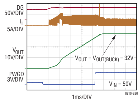
Pass-Thru Start-Up: V_{IN} Above Pass-Thru Window (Figure 38)
