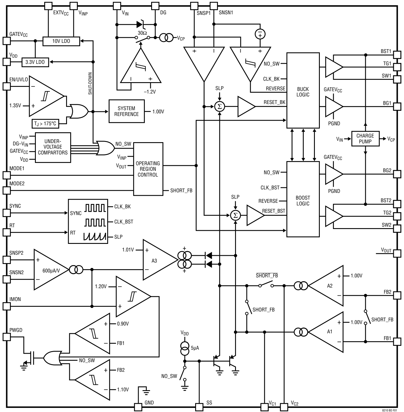
Figure 1. Block Diagram
