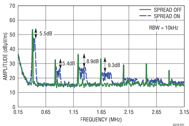
Figure 21. Conducted Average EMI Comparison (AM Band) Example
