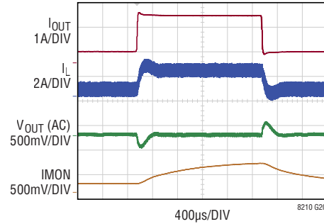
Load Step (Buck-Boost Region – Figure 37)
