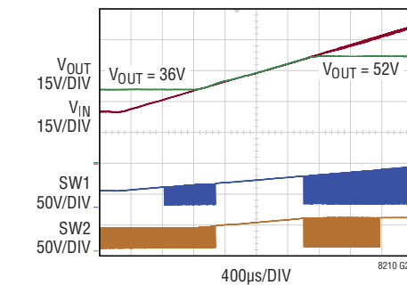
Input Voltage Sweep (Pass-Thru – Figure 37)
