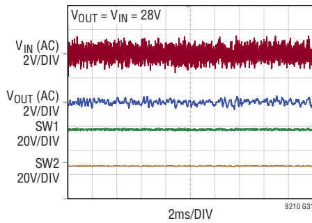
Pass-Thru Regulation with Noisy Input Supply (Figure 38)
