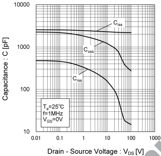
Fig.16 Typical Capacitances vs. Drain - Source Voltage
