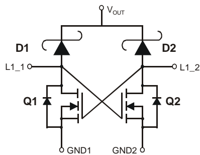
Device Schematic (Dual Channel)
