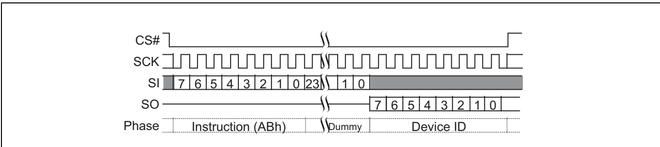
Figure 49 Read electronic signature (RES ABh) command sequence
