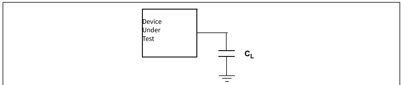
Figure 25 Test setup
