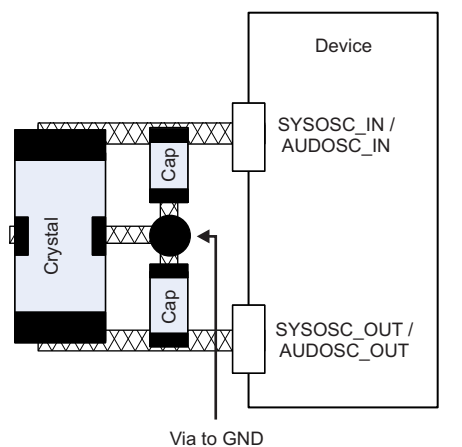
Figure 7-25. SYSOSC and AUDIOOSC PCB requirements
