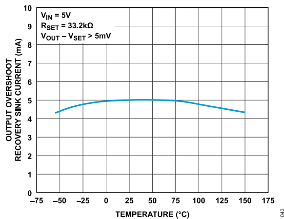
Figure 43. Output Overshoot Recovery Sink Current vs. Temperature
