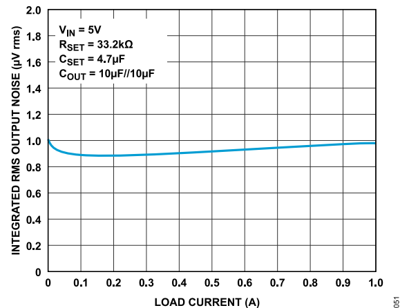
Figure 51. Integrated RMS Output Noise (10 Hz to 100 kHz) vs. Load Current
