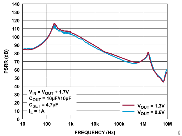
Figure 50. PSRR as a Function of an Error-Amplifier Input Pair vs. Frequency
