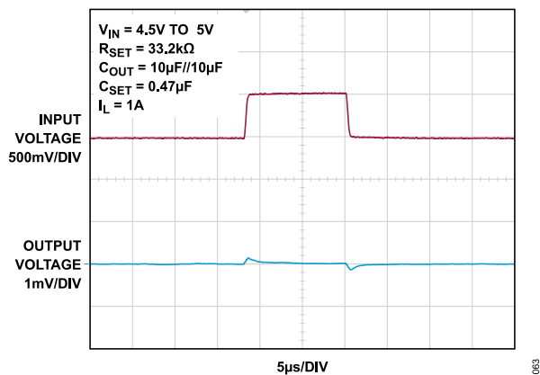
Figure 63. Line-Transient Response
