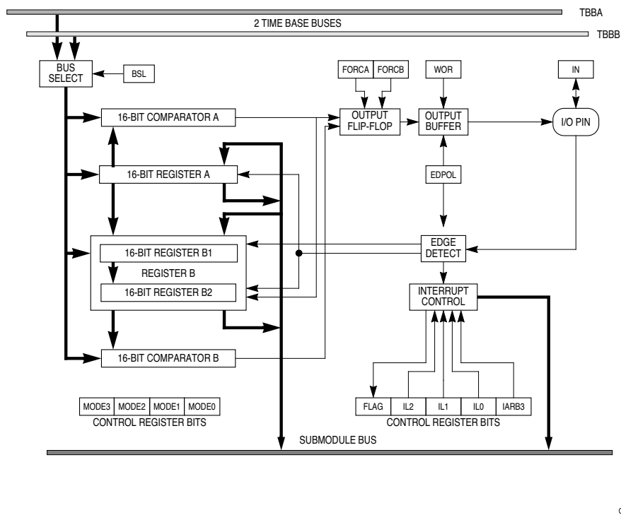
Figure 10-5 DASM Block Diagram
