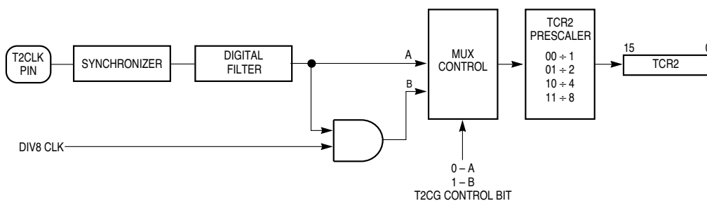
Figure 11-3 TCR2 Prescaler Control
