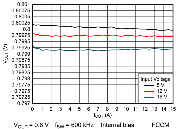
Figure 8-12. Load Regulation
