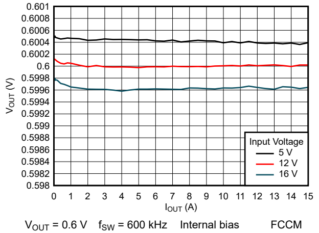
Figure 8-11. Load Regulation
