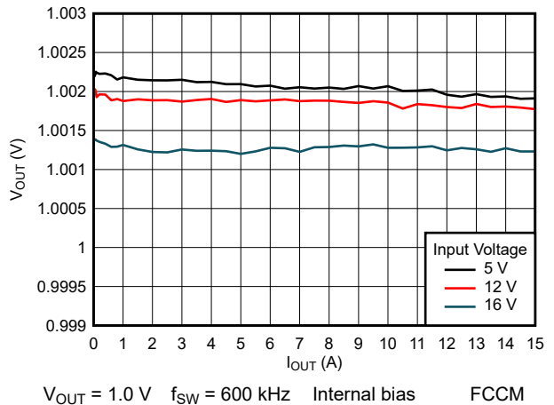
Figure 8-13. Load Regulation
