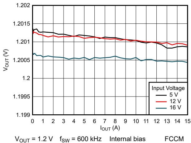
Figure 8-14. Load Regulation
