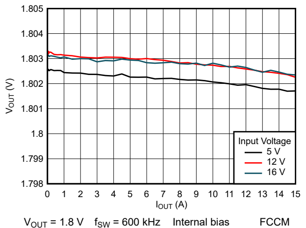
Figure 8-15. Load Regulation
