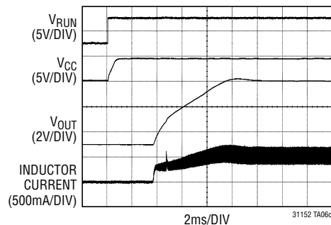
Soft-Start Waveform, V IN = 24V, I LOAD = 0.5A
