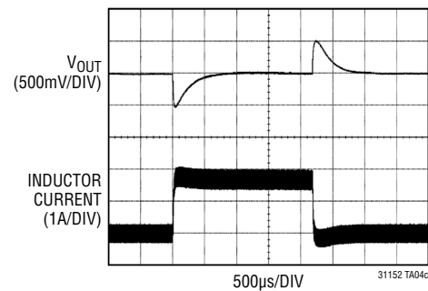
0A to 1.5A Load Step, V IN = 24V
