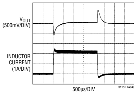
0A to 1.5A Load Step, V IN = 10.6V
