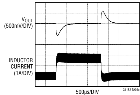
0A to 1.5A Load Step, V IN = 40V
