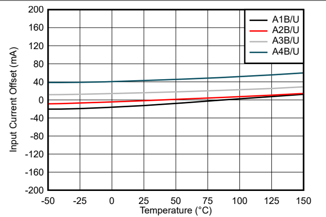
Figure 7-2. TMCS1108 Input Offset Current vs. Temperature
