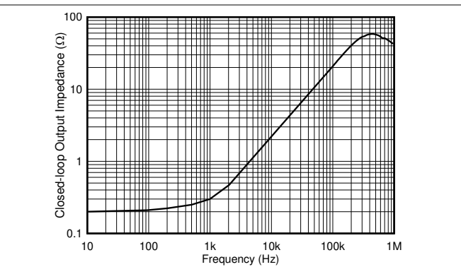
Figure 7-6. Output Impedance vs. Frequency
