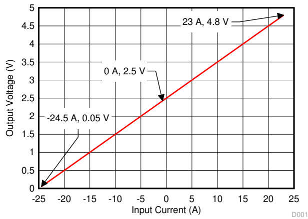
Figure 10-3. Application Example Design Transfer Curve
