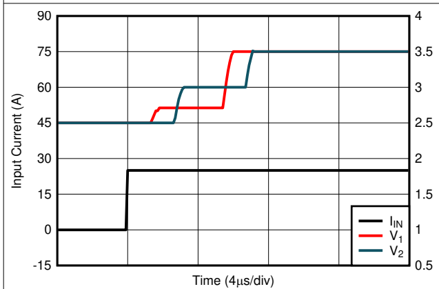
Figure 7-9. Voltage Output Step, Rising
