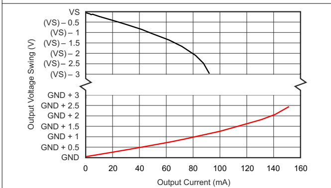
Figure 7-5. Output Swing vs. Output Current
