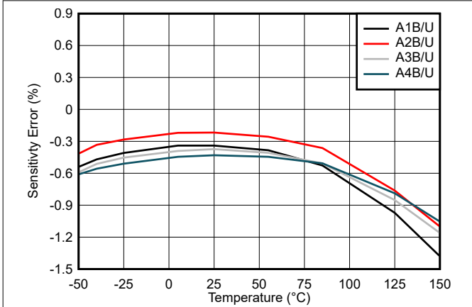
Figure 7-1. TMCS1108 Sensitivity Error vs. Temperature
