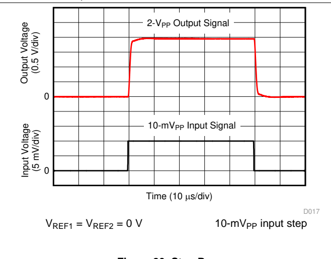
Figure 20. Step Response
