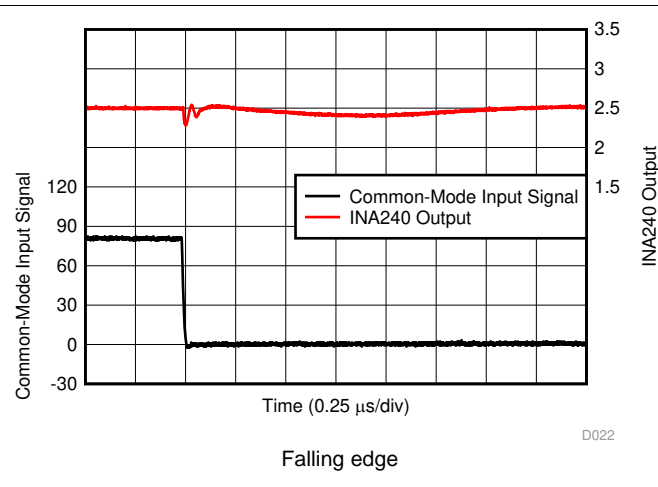
Figure 22. Common-Mode Voltage Transient Response
