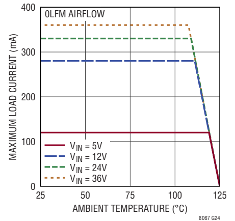
Derating, 3.3V V_{OUT}
