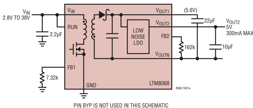
2kVAC Isolated Low Noise μModule Regulator
