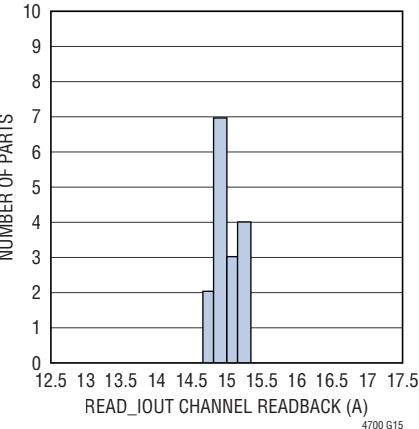
READ_IOUT of 16 LTM4700 Channels 12\text{V}_{\text{IN}} , 1\text{V}_{\text{OUT}} , T_J = 120^{\circ}\text{C} , I_{\text{OUT}} = 15\text{A} , System Having Reached Thermal Steady- State Condition, No Airflow
