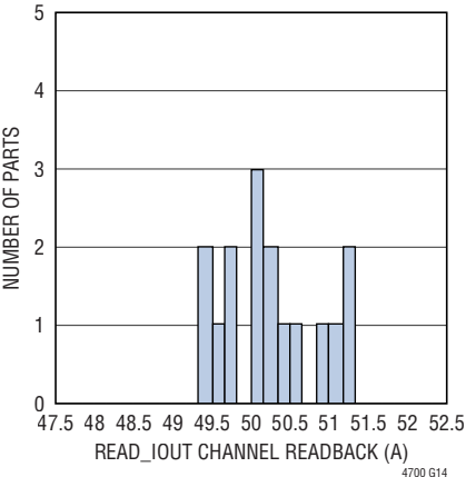
READ_IOUT of 16 LTM4700 Channels 12\text{V}_{\text{IN}} , 1\text{V}_{\text{OUT}} , T_J = 80^{\circ}\text{C} , I_{\text{OUT}} = 50\text{A} , System Having Reached Thermal Steady- State Condition, No Airflow
