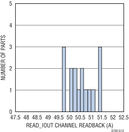
READ_IOUT of 16 LTM4700 Channels 12\text{V}_{\text{IN}} , 1\text{V}_{\text{OUT}} , T_J = -10^{\circ}\text{C} , I_{\text{OUT}} = 50\text{A} , System Having Reached Thermal Steady- State Condition, No Airflow
