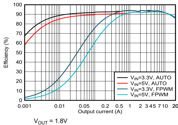
Figure 9-12. Efficiency in 2.2 MHz 4-Phase Mode
