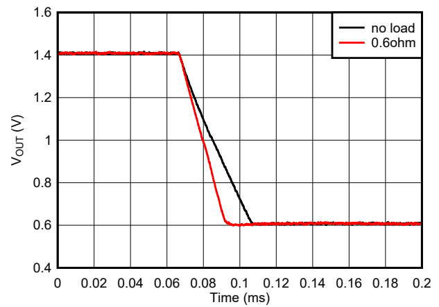
Figure 7-8. Buck Ramp-down Slew Rate
