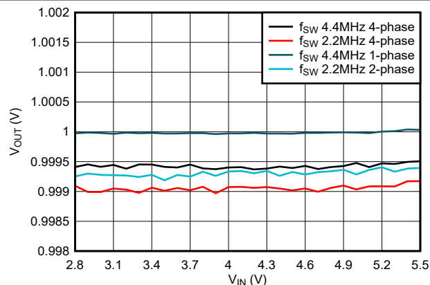
Figure 9-22. Line Regulation
