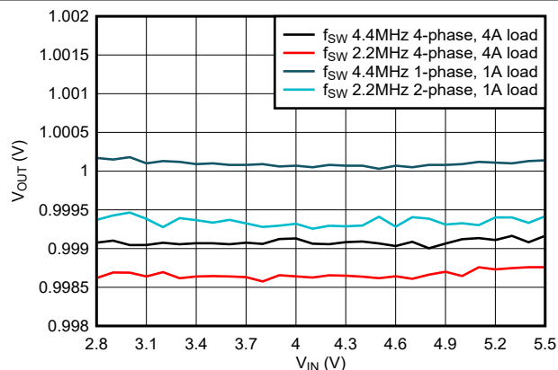
Figure 9-23. Line Regulation
