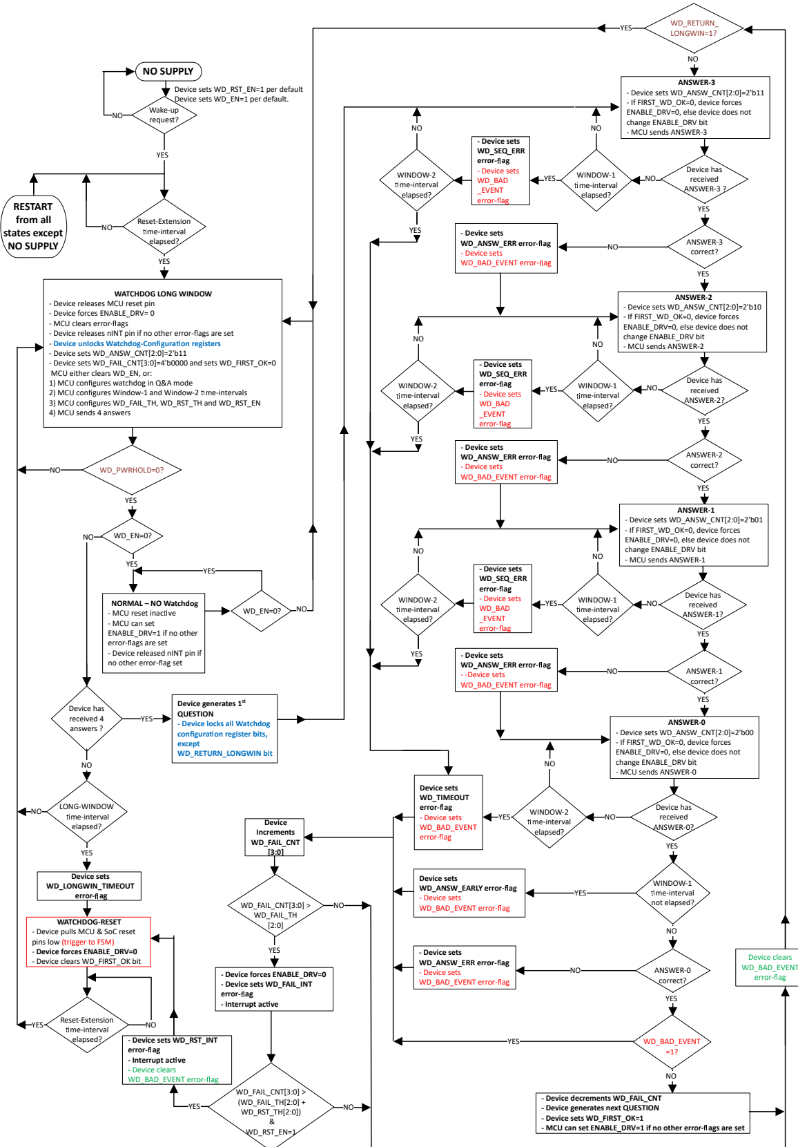
Figure 8-50. Flow Chart for WatchDog in Q&amp;A Mode
