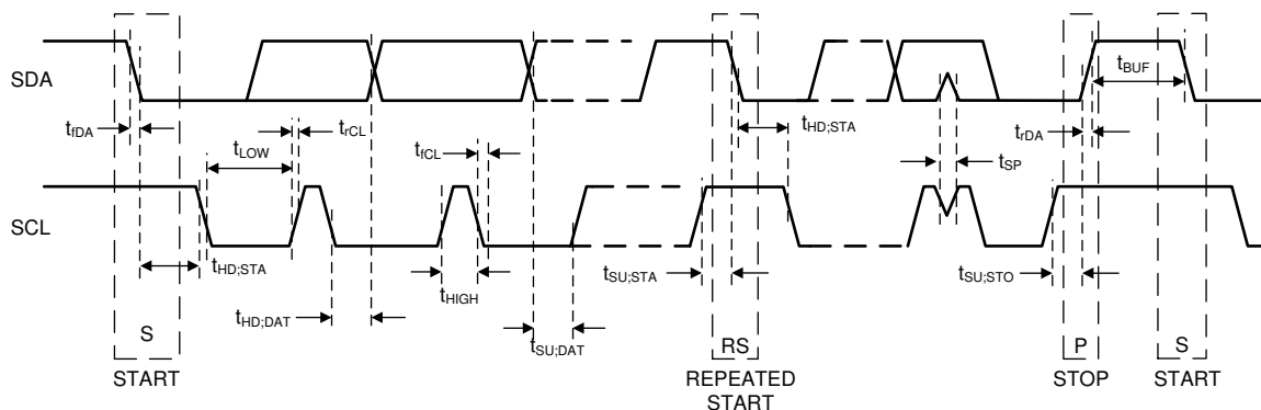
Figure 7-1. I²C Timing
